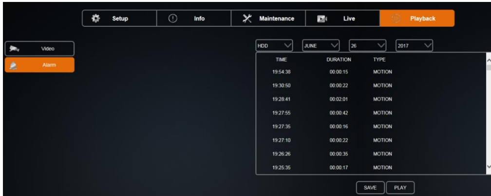
Figure 75: Alarm Tab - Alarm Search
