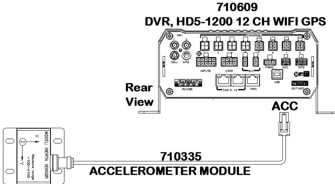
Figure 11: Accelerometer Module Harness Connection
