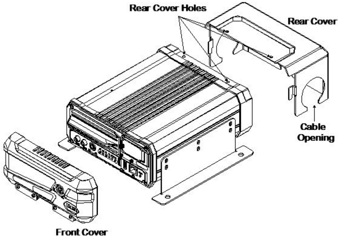
Figure 15: Security Cover Mounting
