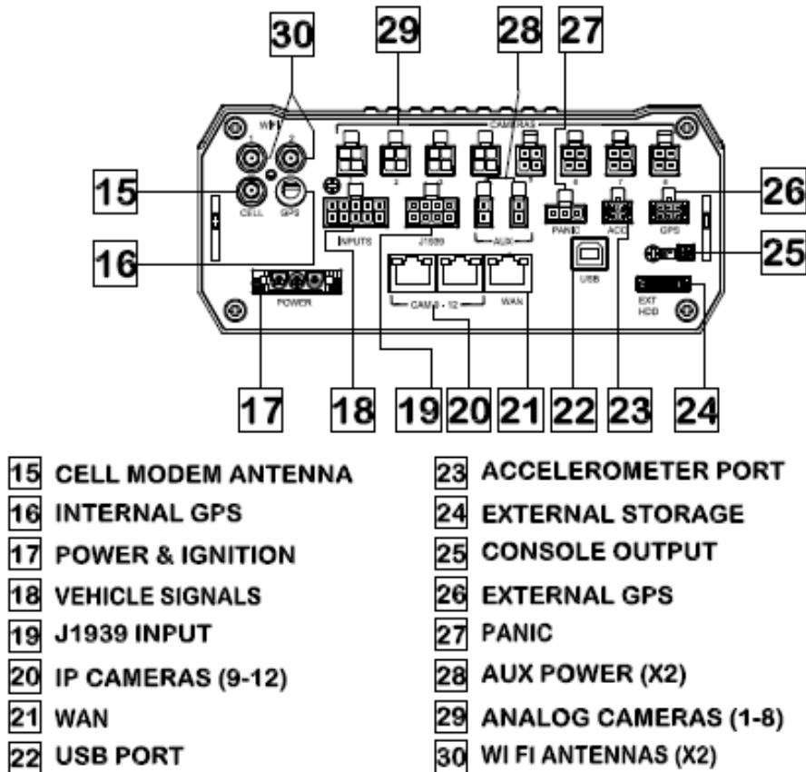
Figure 3: Rear Panel Layout
