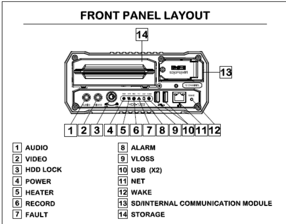
Figure 2: Front Panel Layout
