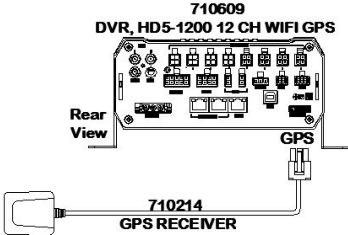
Figure 9: GPS Antenna Module Harness Connection
