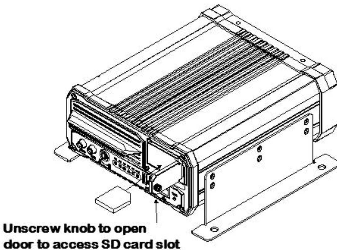
Figure 5: Removable SD Card
