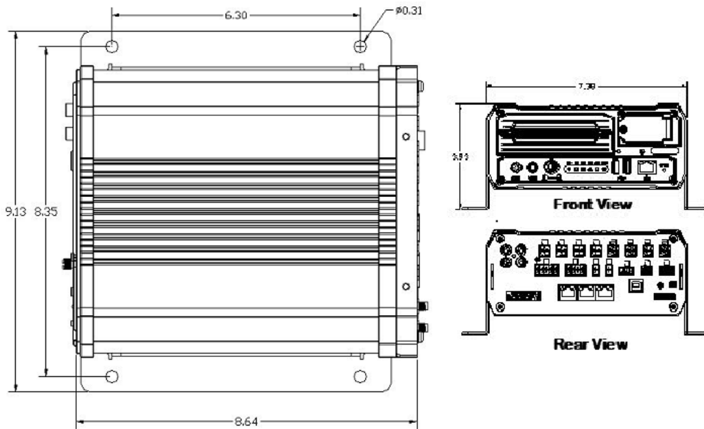
Figure 14: DVR Dimensions
