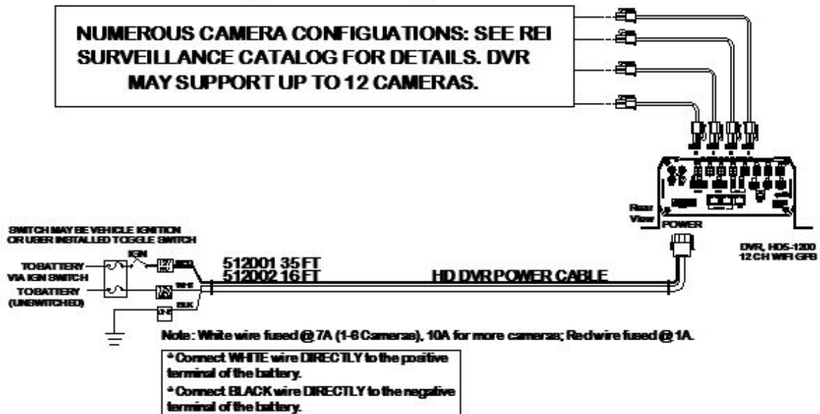
Figure 7: System Wiring - Power and Camera Cables
