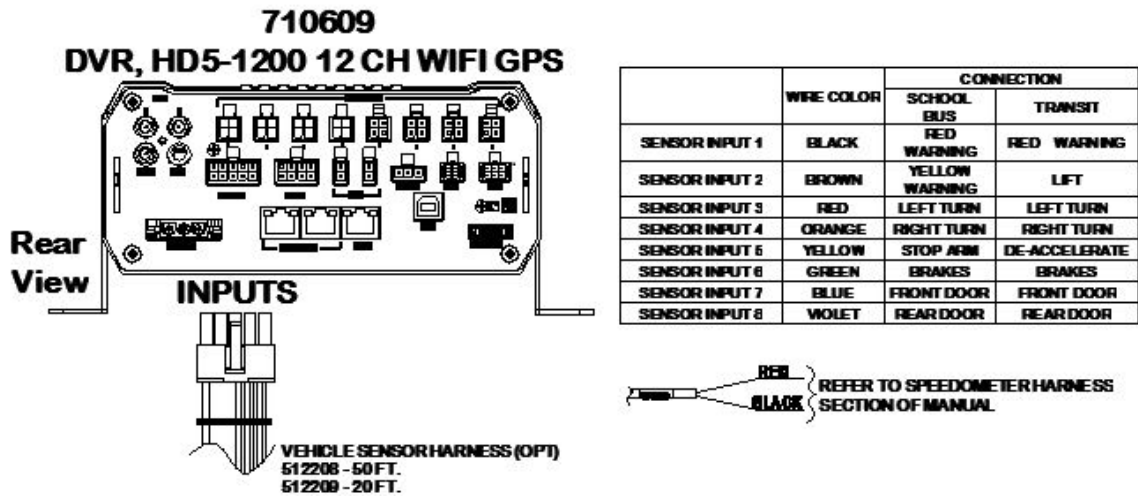
Figure 10: Vehicle Sensor Options Harness Connection
