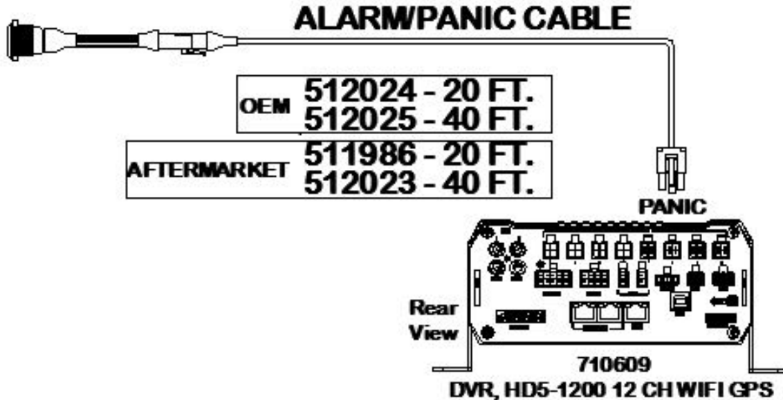
Figure 8: External Record Indicator/Event Mark Button Harness Connection
