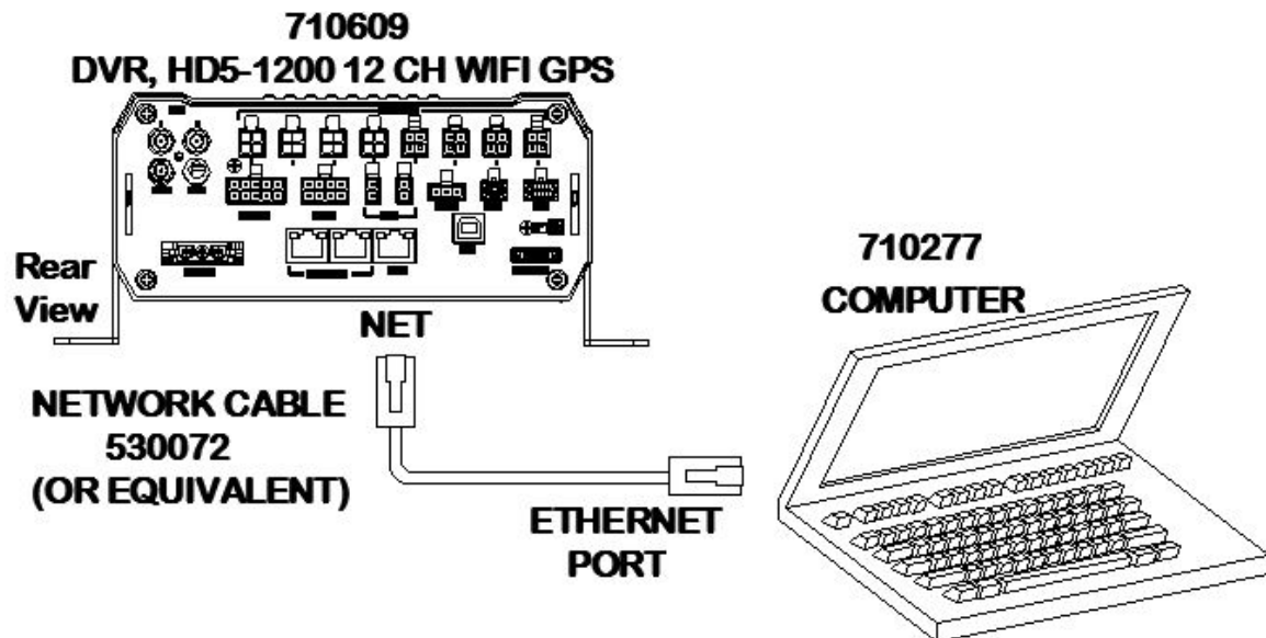
Figure 16: Connecting to the DVR with a Computer through the Ethernet Connection
