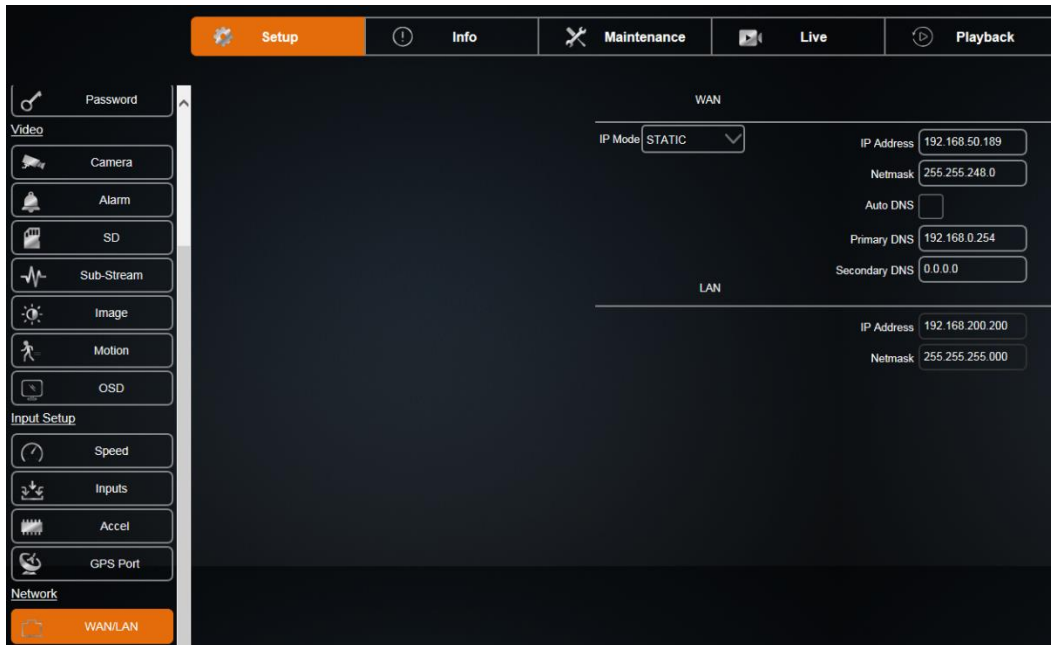
Figure 51: General Network Setup
